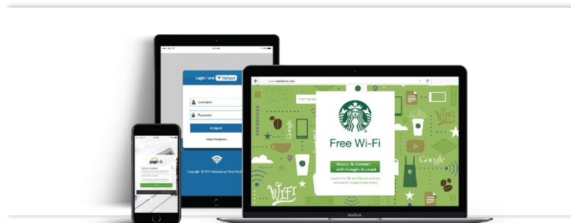
Captive Portal
